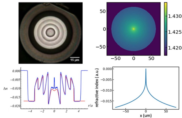
Figure 9. (top left) Optical micrograph of the Airy fiber (bottom left) physical refractive index profiles of the designed Airy (red), and of that of the PCVD preform (blue). Reproduced from I. Gris-Sánchez et al [161], (CC-BY 4.0). (top right) 2D theoretical refractive index profile of a fiber with logarithmic profile. (bottom right) 1D refractive index profile of the same fiber (relative to undoped silica). Reproduced from [161]. CC BY 4.0.
